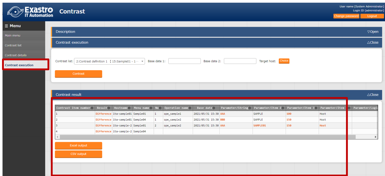
Figure 5.1-7 Compare execution screen (Compare results)
